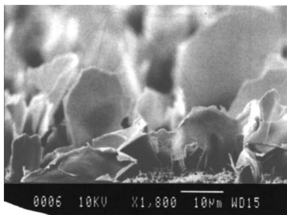
Figure 5. SEM photo of InP etched with \text{BCl}_3/\text{Ar} and excess oxygen.
