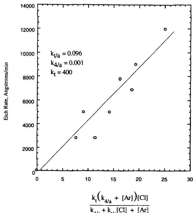
Figure 11. Experimental data plotted in the form of the rate law.
