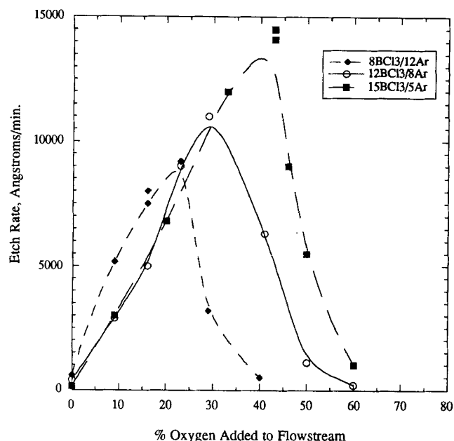
Figure 4. Effect of oxygen addition for different \text{BCl}_3/\text{Ar} gas mixtures on InP etch rate at 250^\circ\text{C} .
