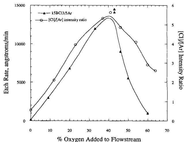
Figure 7. Comparison of InP etch rate and chlorine intensity as a function of oxygen addition.
